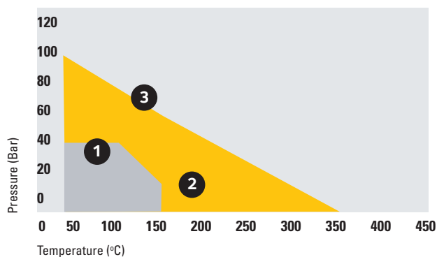
SF 2401 Pressure/Temperature Limits
